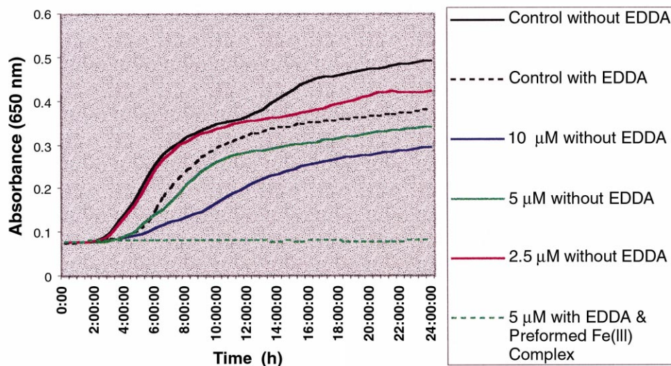
Figure 6. Growth curves of E. coli X580 in Luria broth in the presence of bis-val-5FU conjugate 22 .
