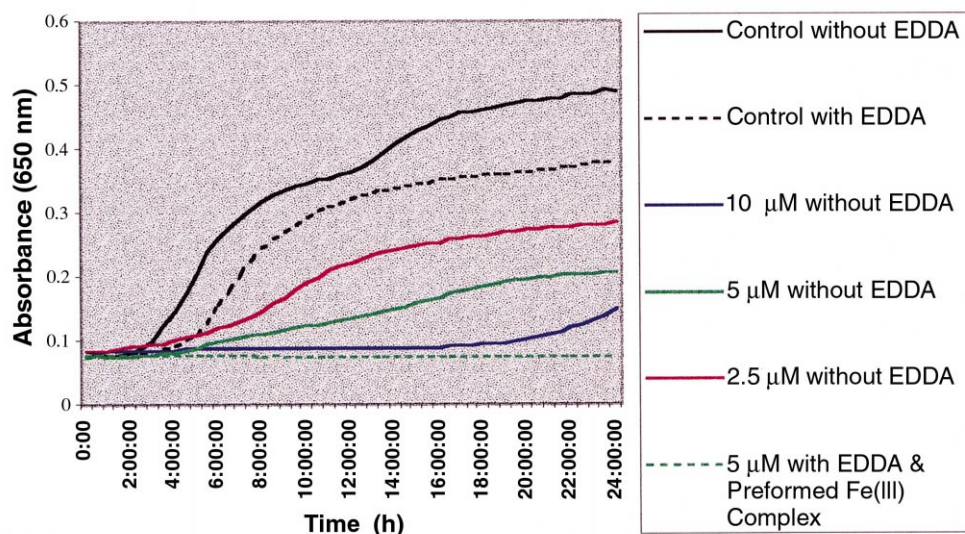
Figure 5. Growth curves of E. coli X580 in Luria broth in the presence of tris-val-5FU conjugate 23 .
