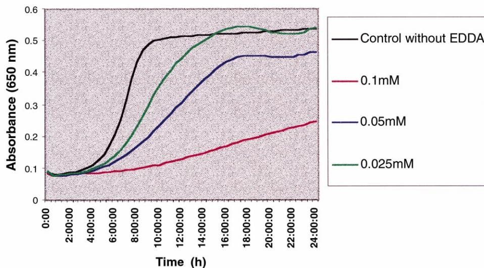
Figure 13. Growth curves of C. albicans in the presence of mono-val-5FU conjugate 21 .
