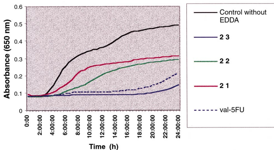
Figure 8. Growth curves of E. coli X580 in the presence of 23 , 22 and 21 and val-5FU at 10 \mu M under regular conditions.
