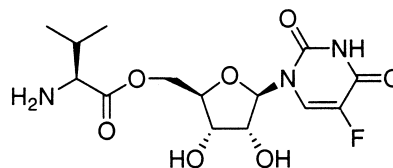
Figure 4. Valine-5-fluorouridine (val-5-FU).
