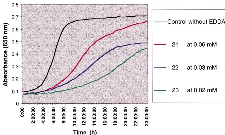
Figure 15. Growth curves of C. albicans in the presence of 21 , 22 and 23 at regular condition.
