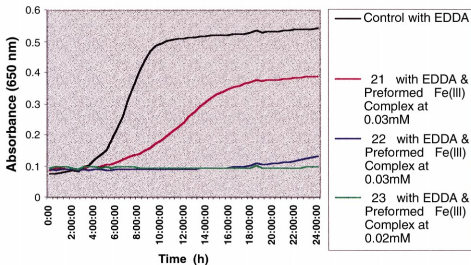
Figure 16. Growth curves of C. albicans in the presence of 21 , 22 and 23 at iron deficient conditions.
