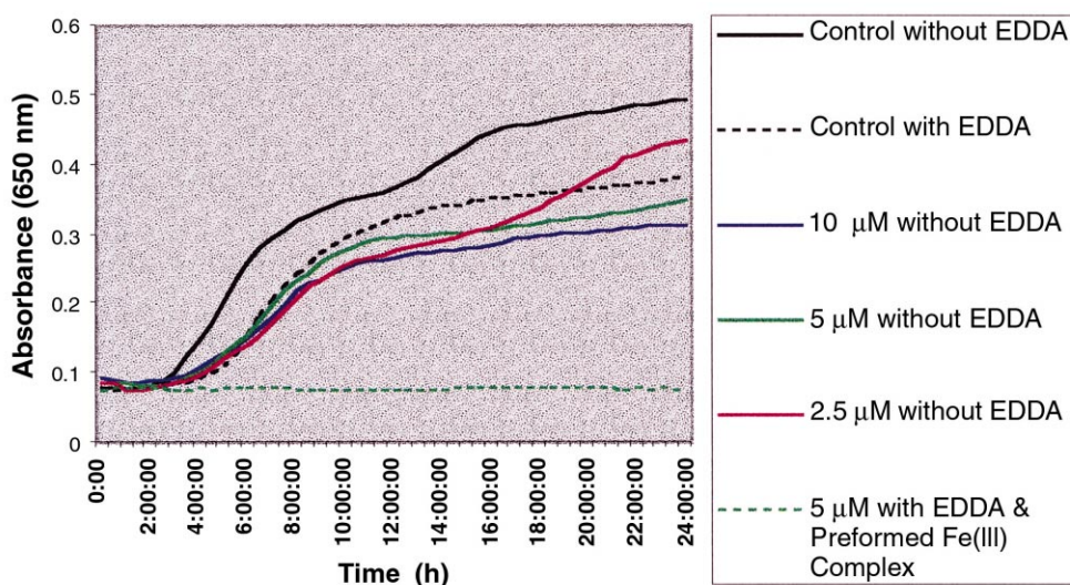
Figure 7. Growth curves of E. coli X580 in Luria broth in the presence of mono-val-5FU conjugate 21 .
