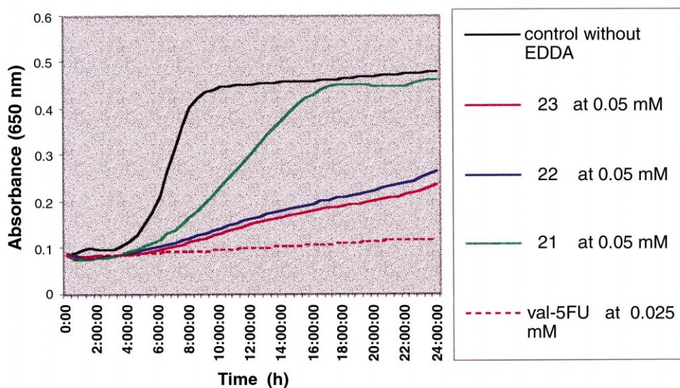
Figure 14. Growth curves of C. albicans in the presence of 21 , 22 and 23 and val-5FU.
